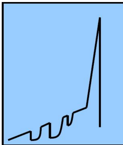
Figure B.4 – Sudden Drops in Torque in Thread/Seal Interference Possible Causes: Tong and/or backup dies are slipping.
