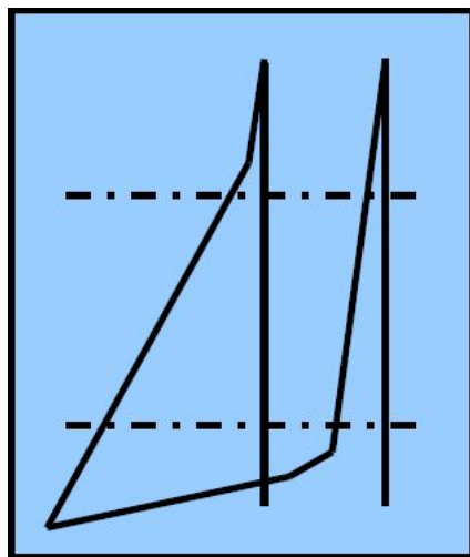
Figure B.3 – Connection Shoulders above the maximum allowed torque or under the minimum allowed torque Possible Causes: misalignment, poor calibration
